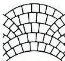
EUROPEAN FAN BRICK SIZE: RANDOM ROLL WIDTH: 33" JOINT WIDTH: 1/2" - 1 1/2"
