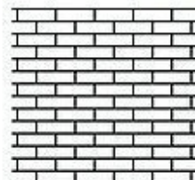
FACE BRICK BRICK SIZE: 2 1/2" X 7 1/2" ROLL WIDTH: 36 1/2" JOINT WIDTH: 1/4"
